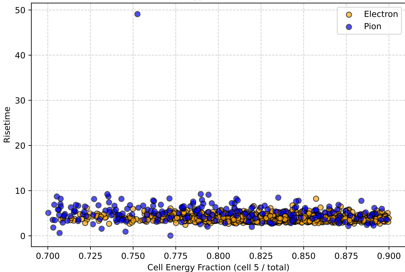
Risetime vs Cell Energy Fraction for 1.0GeV particles
